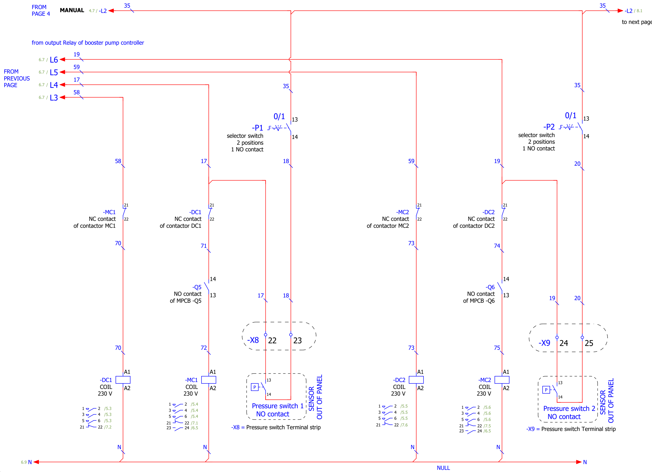
Control circuit diagram 1
