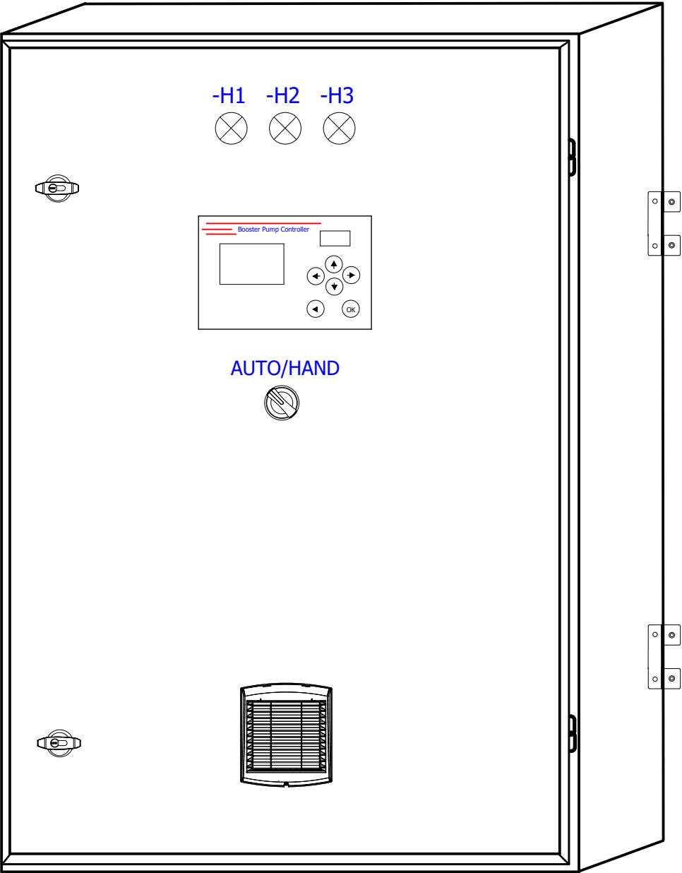
EXTERNAL VIEW
