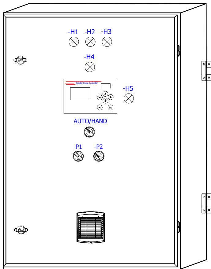
EXTERNAL VIEW
