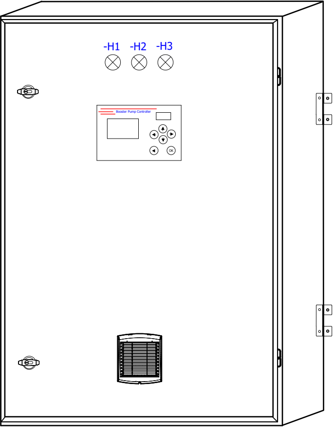
EXTERNAL VIEW
