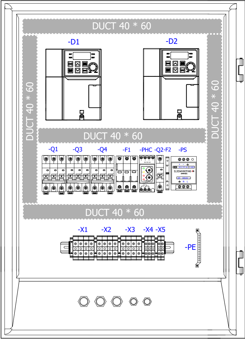
INTERNAL VIEW
