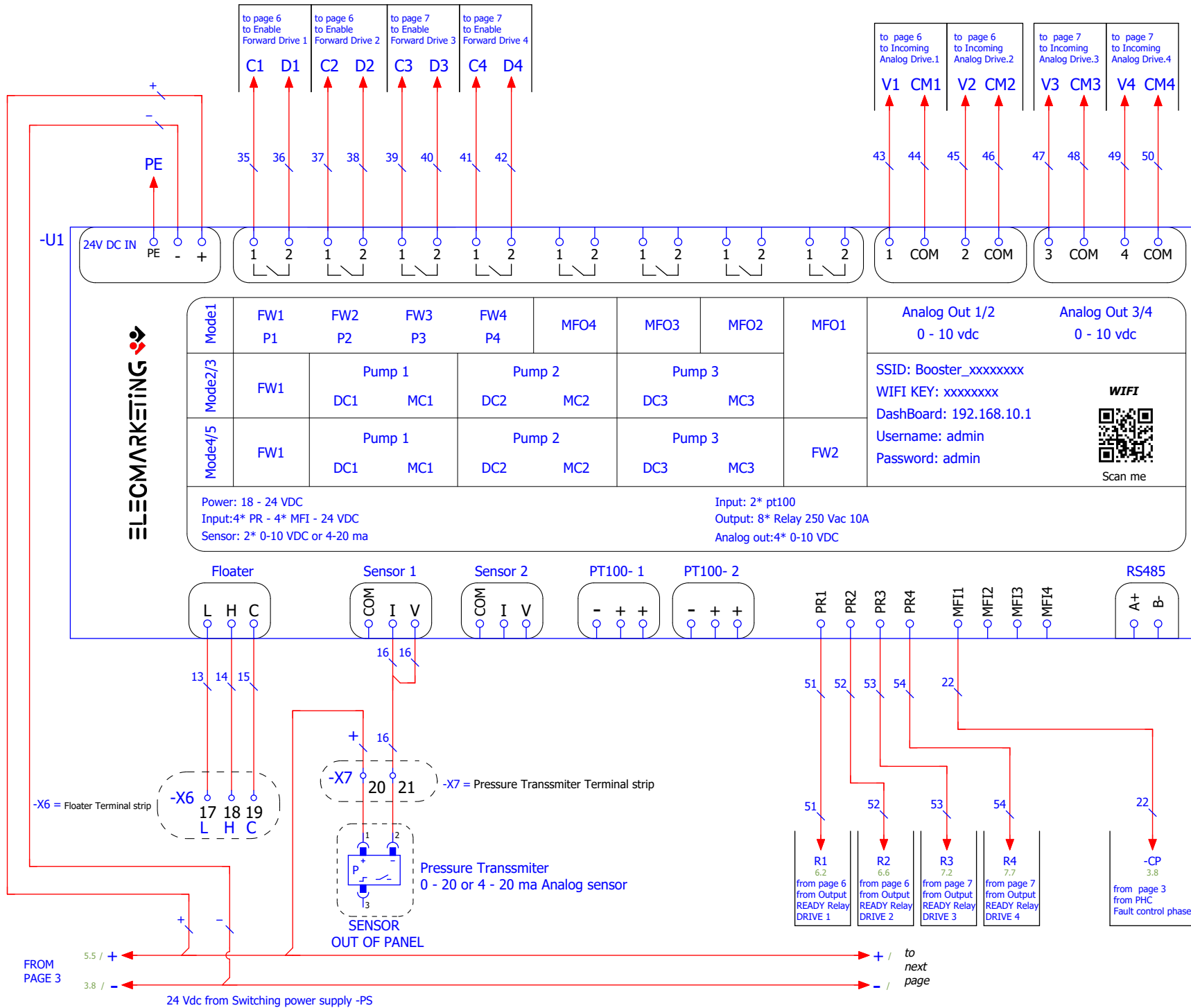
Controller schematic diagram
